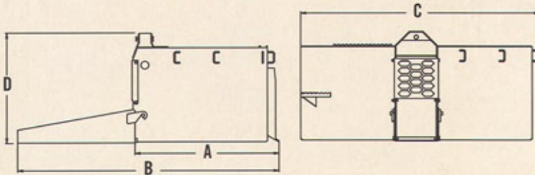
1/2 yd Concrete Chuter
